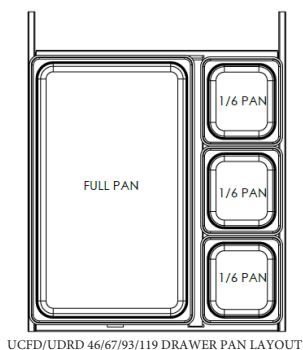
UCRD/UDRD 46/67/93/119 DRAWER PAN LAYOUT
